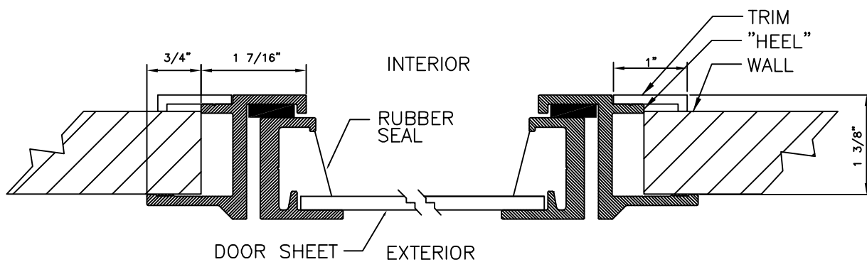
SECTION A
