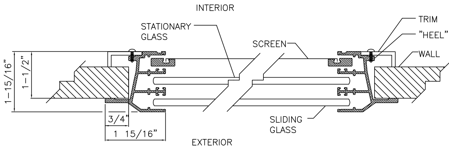
SECTION A
