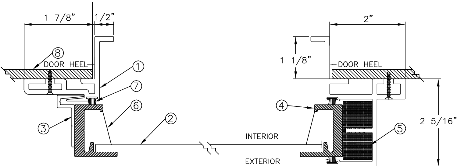
SECTION A
